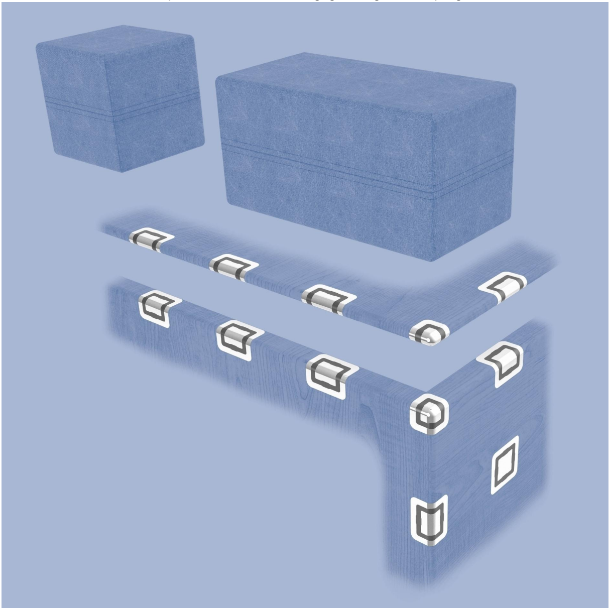
Perspective view of the disengaged magnetic couplings
