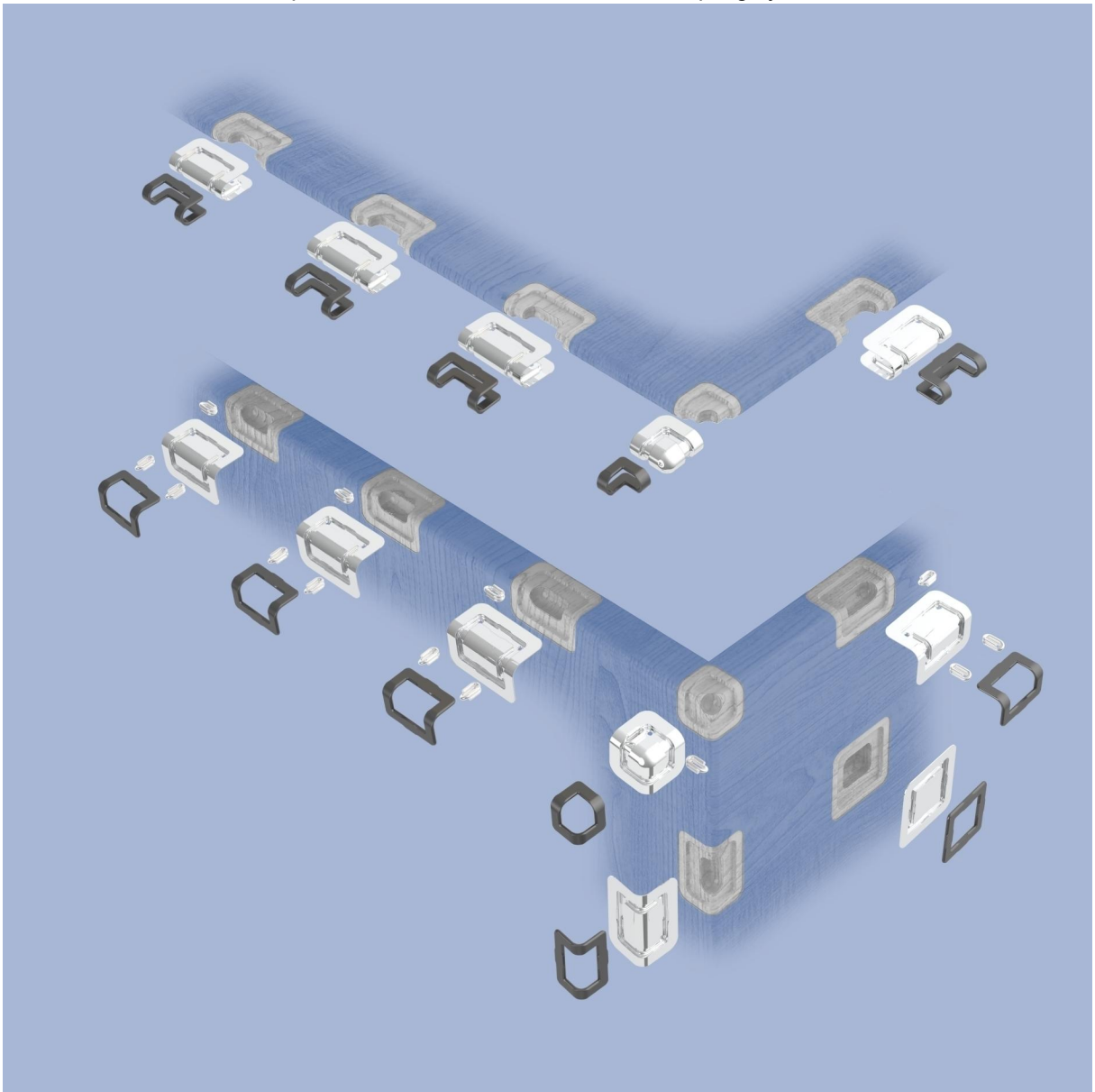
Exploded view of a modular furniture coupling system
